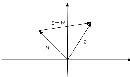
Fig. C.2 Geometry behind the distance of two complex numbers.
